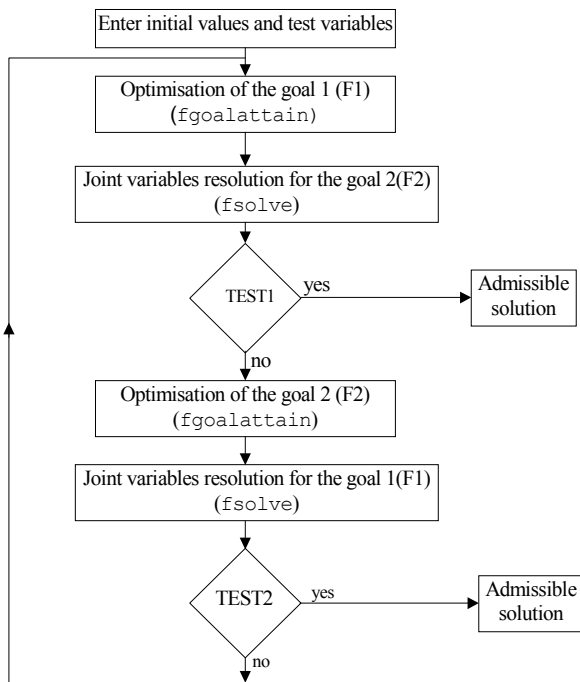
Figure 11. Optimisation algorithm
