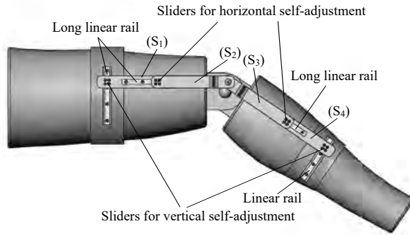
Fig. 5 The simulated self-adjustment mechanism.
