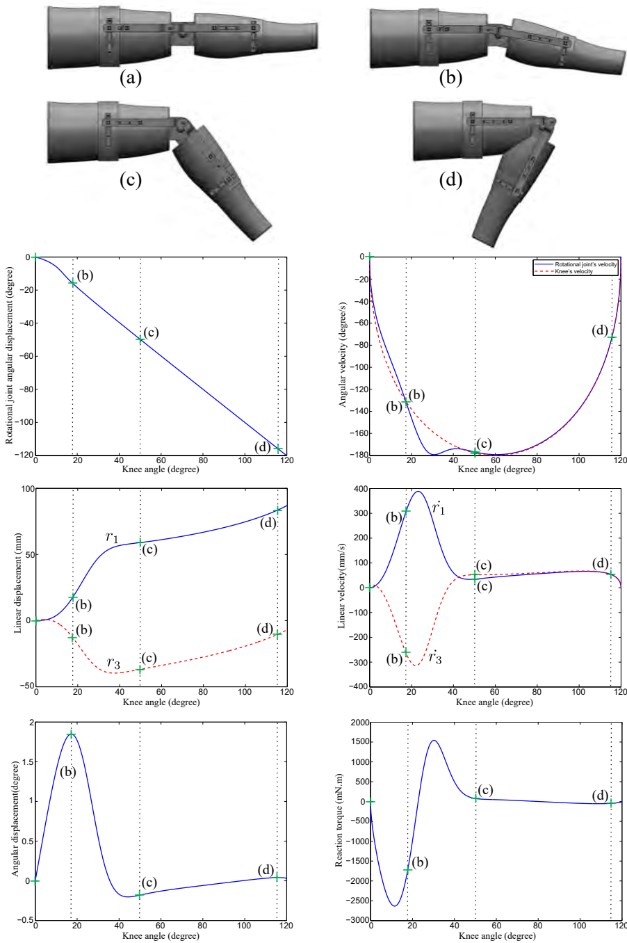
Top: PRP mechanism in different representative configurations. (a) Initial configuration. (b) Configuration before self-adjustment. (c) Configuration just after self adjustment. (d) Final configuration after complete knee flexion. Bottom: (1) Orthosis angle ( \theta_2 ). (2) Orthosis angular velocity ( \dot{\theta}_2 ). (3) Displacement of the sliders 1 and 3. (4) Velocity of the sliders 1 and 3. (5) Angle at the calf attachment ( \theta_4 ). (6) Torque at the calf attachment. The horizontal axis represents the angle of the knee joint.
