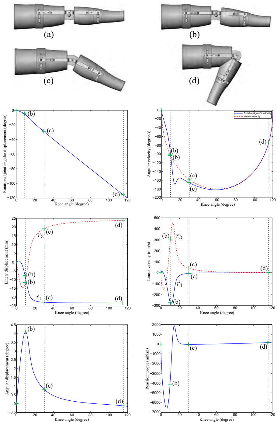
Top: PRP mechanism in different representative configurations. (a) Initial configuration. (b) Configuration during the beginning of self-adjustment. (c) Configuration after self adjustment. (d) Final configuration after complete knee flexion. Bottom: (1) Orthosis angle ( \theta_2 ). (2) Orthosis angular velocity ( \dot{\theta}_2 ). (3) Displacement of the sliders 1 and 3. (4) Velocity of the sliders 1 and 3. (5) Angle at the calf attachment ( \theta_4 ). (6) Torque at the calf attachment. The horizontal axis represents the angle of the knee joint. Letters beside the curves inform on the data values at knee angles corresponding to configurations.
