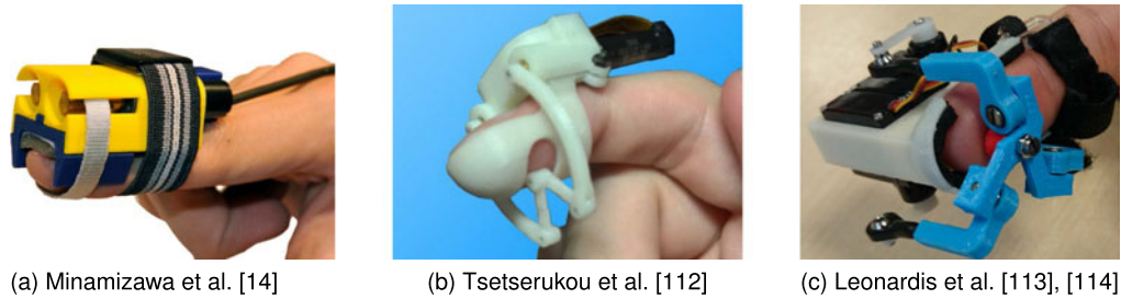
Fig. 3. Three representative wearable haptic devices providing lateral skin stretch and/or relative tangential motion to the fingertip.
